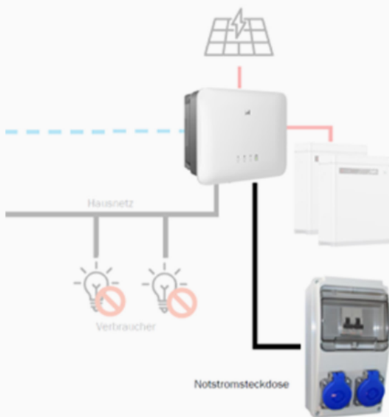
1-phasige Installation
